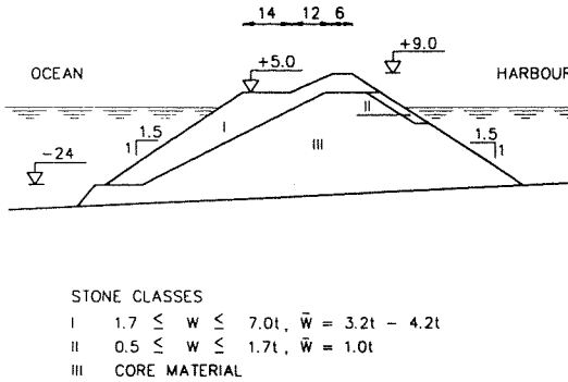
Figure 7 Cross-section of a berm breakwater at Keflavik. (Based on figure from Baird (1987)). All measures are in metres.
