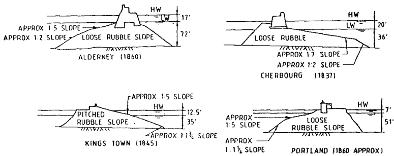
Figure 2 Examples of historical berm breakwaters (Figure from Hall (1987)).
