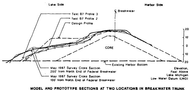
MODEL AND PROTOTYPE SECTIONS AT TWO LOCATIONS IN BREAKWATER TRUNK
