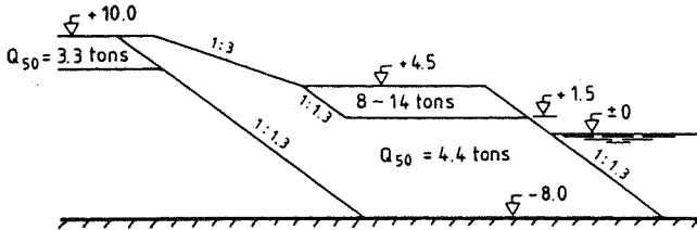
Figure 4 Extension of breakwater at Årviksand, profile of breakwater head, (Figure from Tørum et al (1990)). All measures are in metres.
