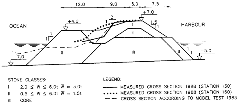
Figure 6 Measurements of profile reshaping of berm breakwater at Bakkafjordur (based on figures from Viggoisson (1990)). All measures are in metres.
