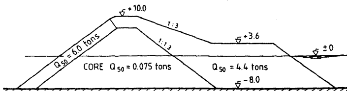
Figure 3 Extension of breakwater at Årvikstrand, profile of breakwater trunk section (Figure from Tørum et al (1990)). All measures are in metres.
