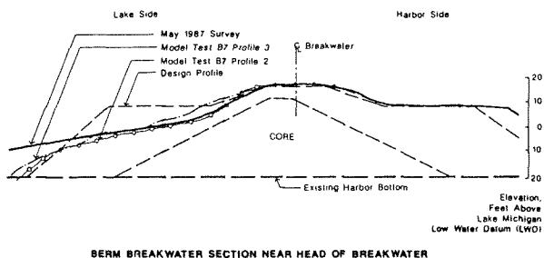
BERM BREAKWATER SECTION NEAR HEAD OF BREAKWATER
