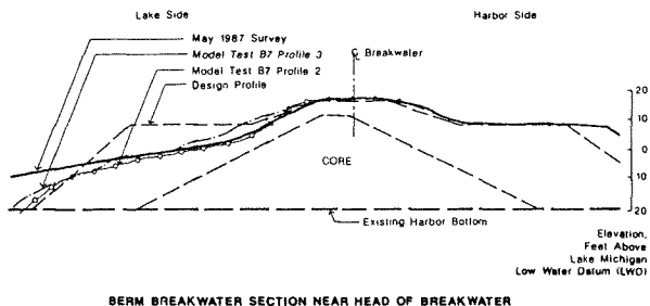
Figure 13 Comparison of model tests and prototype measurements. (Figures from Montgomery et al (1987)). All measures are in feet.
